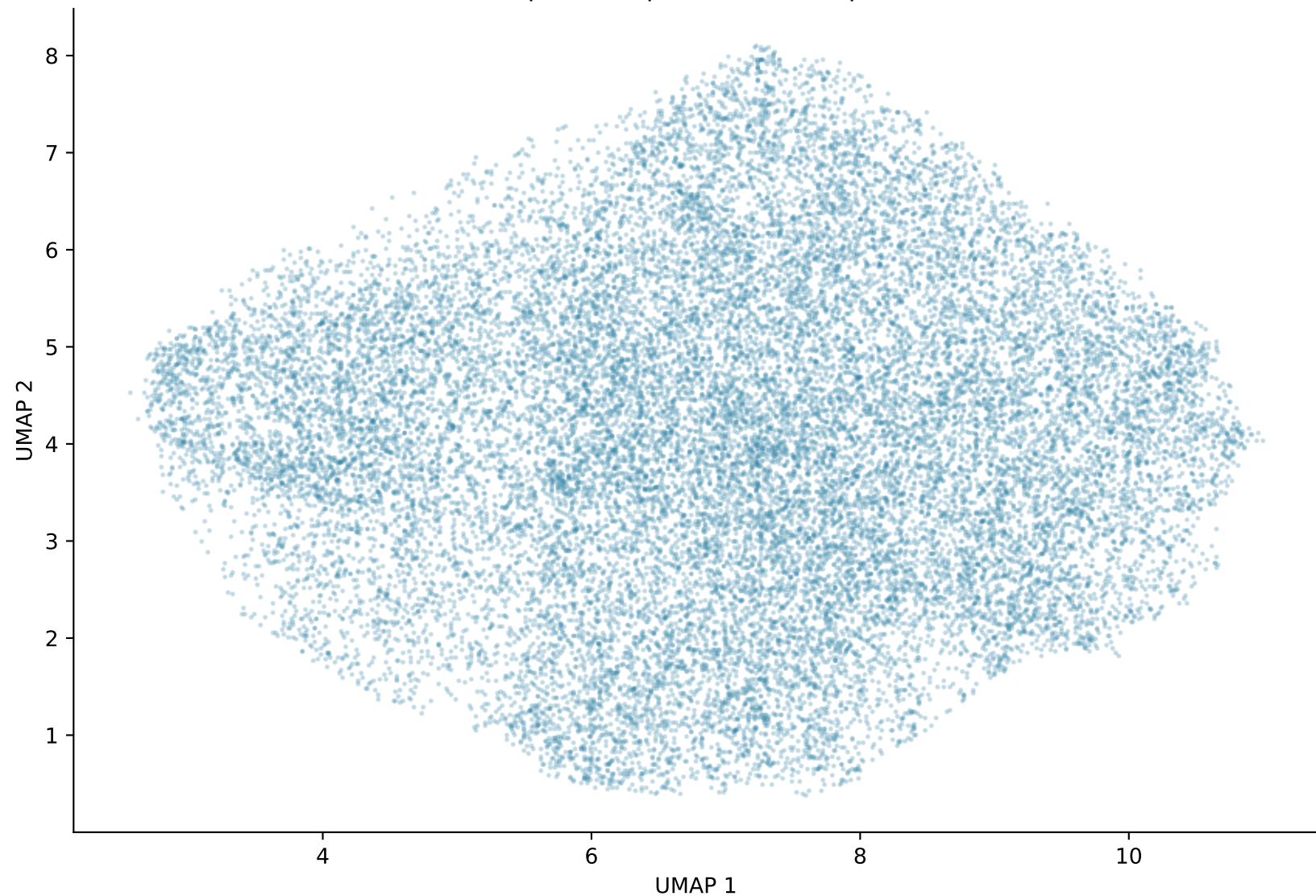
Image Graph Descriptors: UMAP (n=378,818; plot sample=24,000) raw 2080D descriptors; n_neighbors=30, min_dist=0.15, metric=euclidean Graph descriptors in UMAP space
