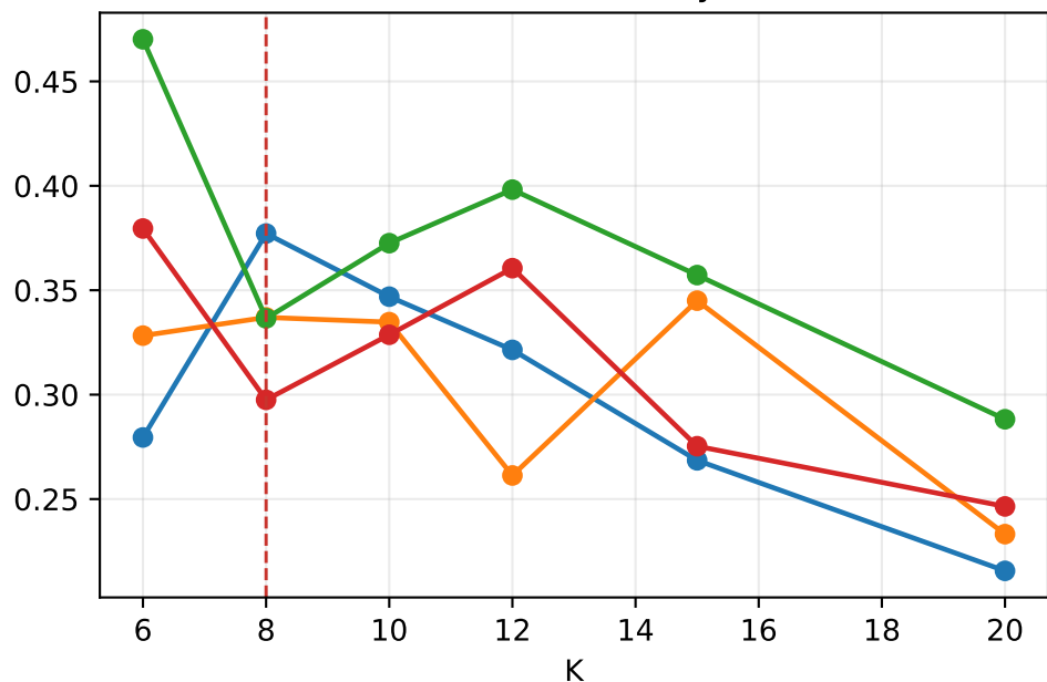
Composite selection score
