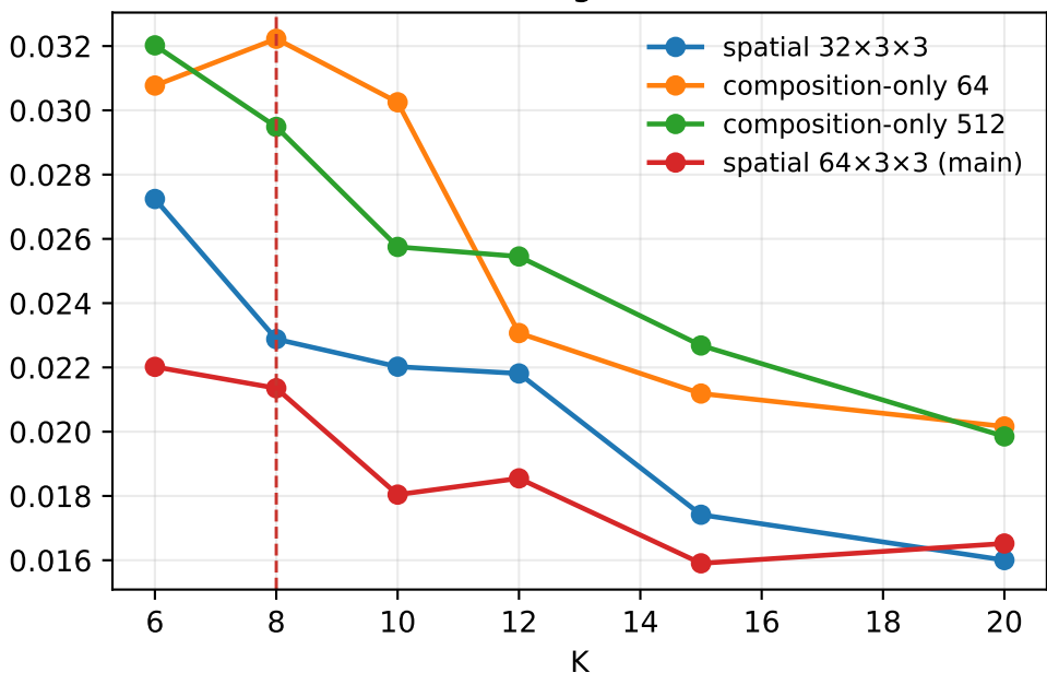
Smallest archetype share
