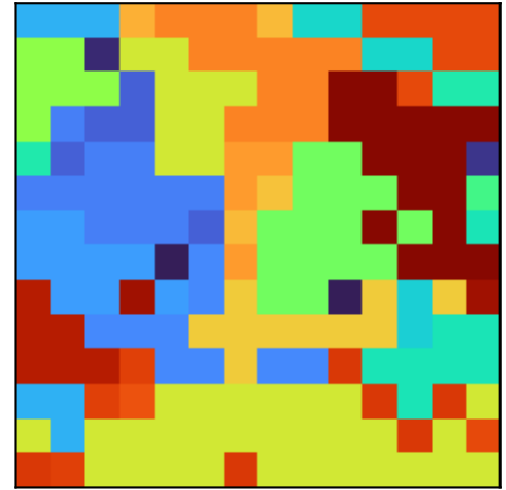
Image graph
