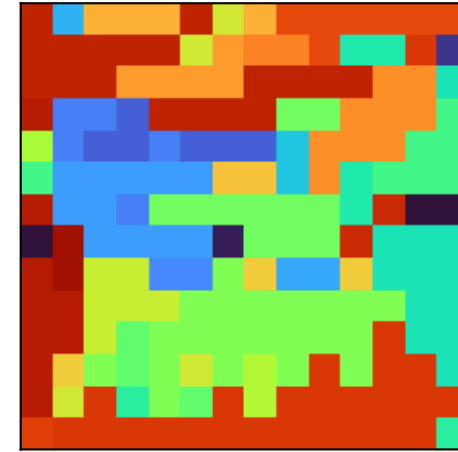
Image graph
