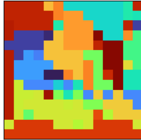
Image graph
