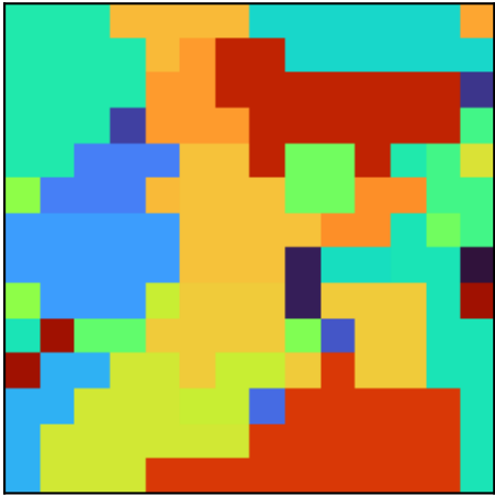
Image graph
