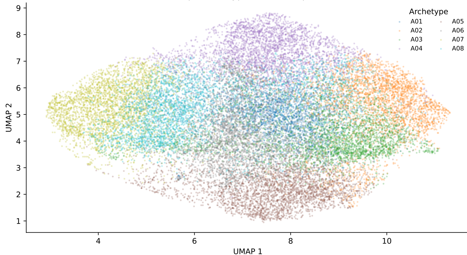
Image Graph Archetypes: UMAP and K=8 clustering (n=378,818; plot sample=24,000) raw 2080D descriptors; n_neighbors=30, min_dist=0.15, metric=euclidean Graph archetypes in UMAP space
