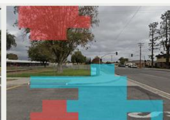
LosAngeles 29/28 patches
