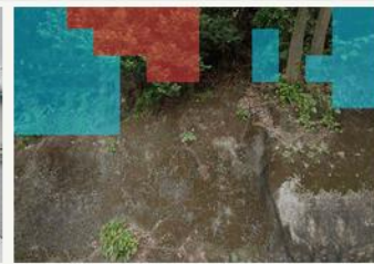
HongKong 20/33 patches
