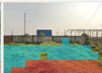
Dhaka 48/29 patches
