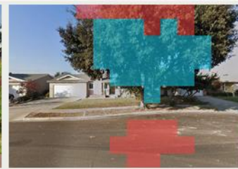
LosAngeles 25/24 patches
