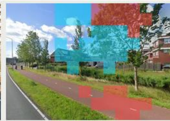
Amsterdam 25/24 patches
