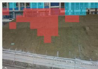
HongKong 24/30 patches
