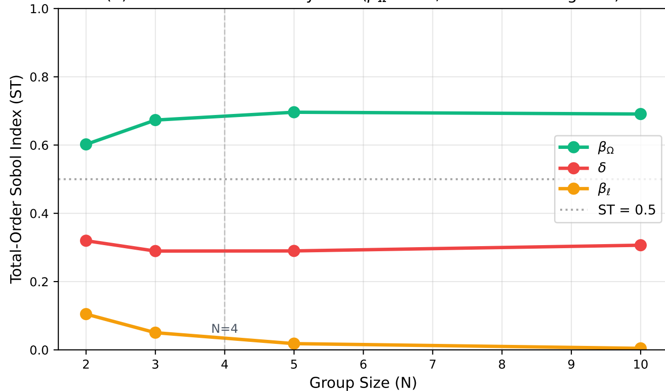
(a) Total-Order Sensitivity vs N ( \beta_\Omega leads, \delta second throughout)
