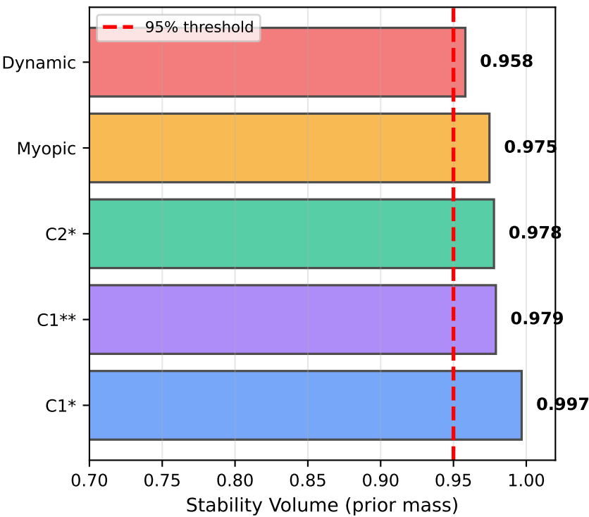
(2) Overall Robustness
