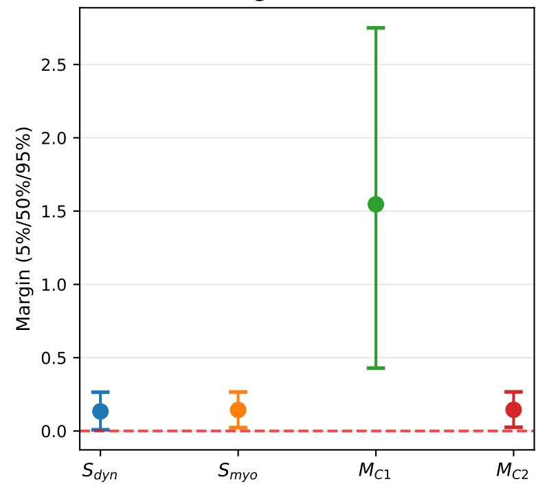
(4) Margin Distributions
