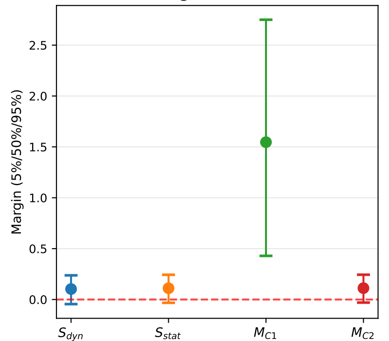
(4) Margin Distributions
