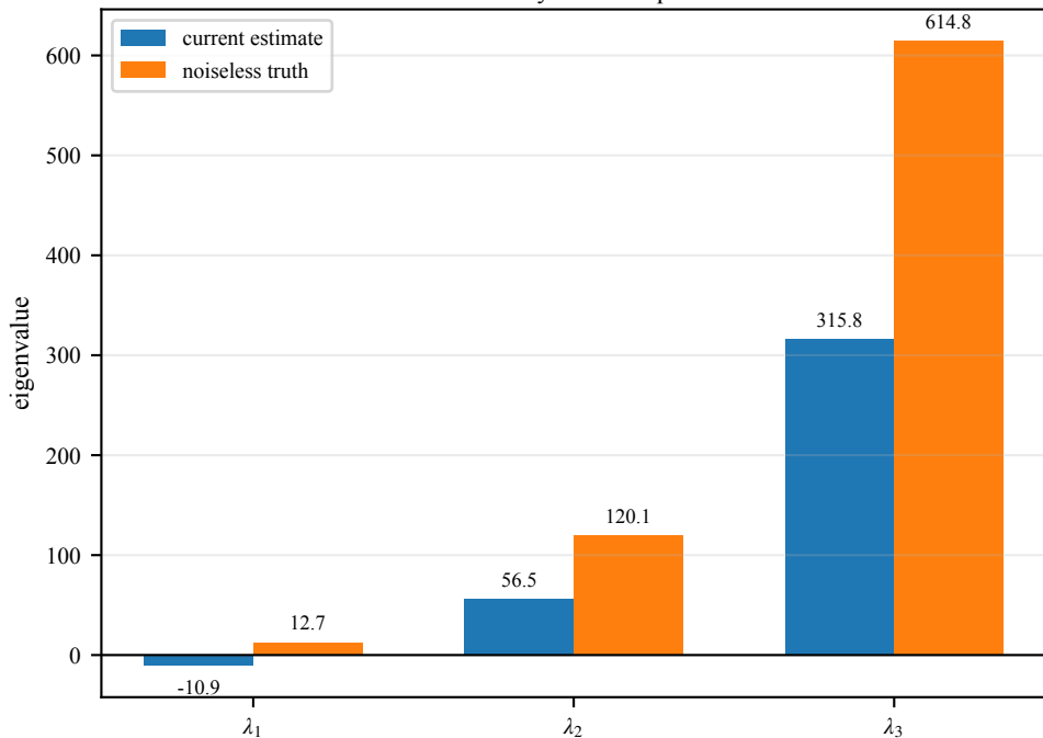
Rotation-only Hessian spectrum
