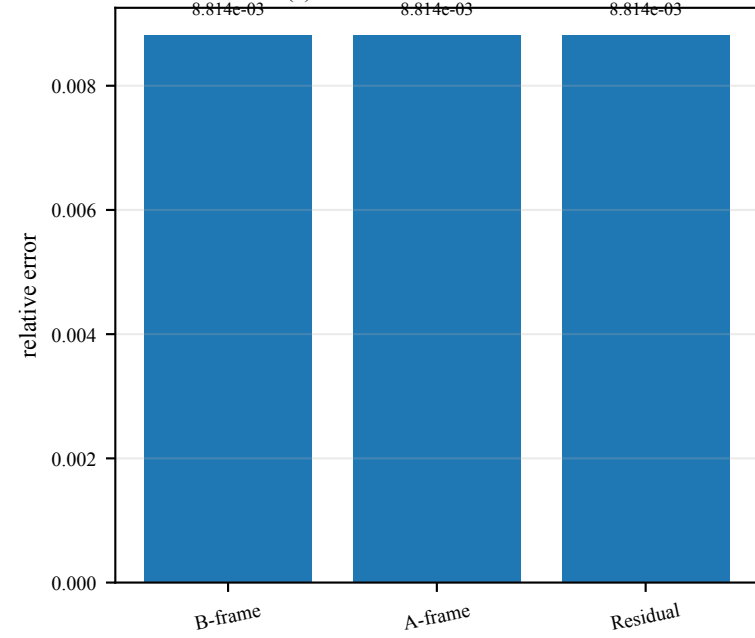
(a) Total Jacobian relative error
