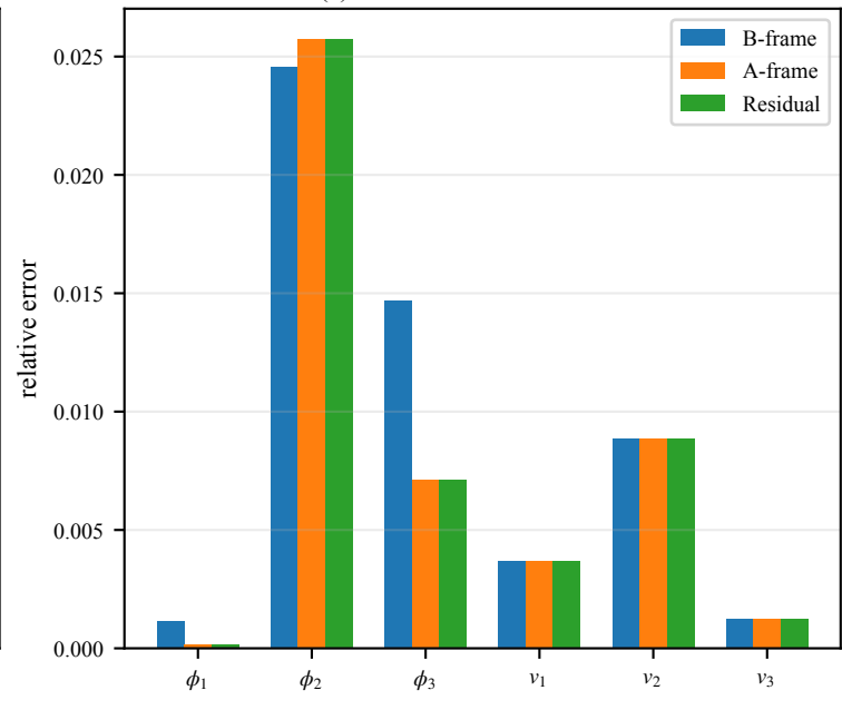
(c) Column-wise relative error
