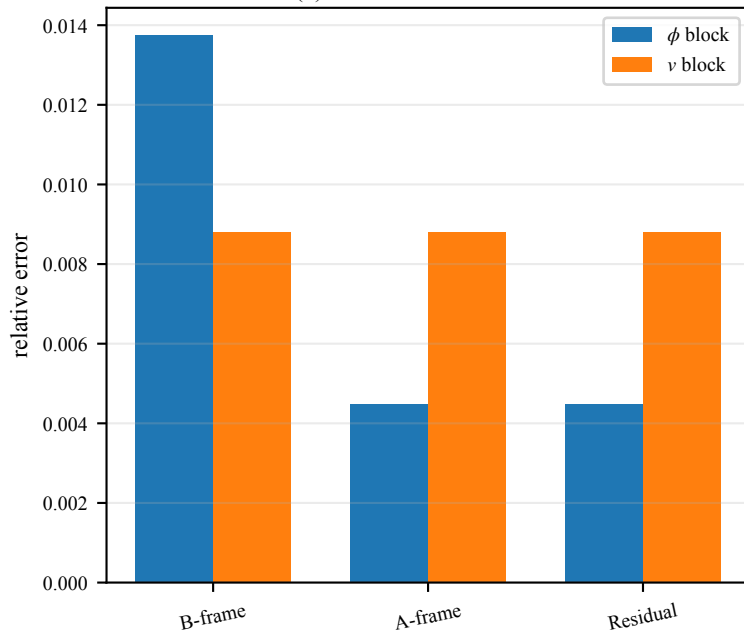
(b) Blockwise relative error
