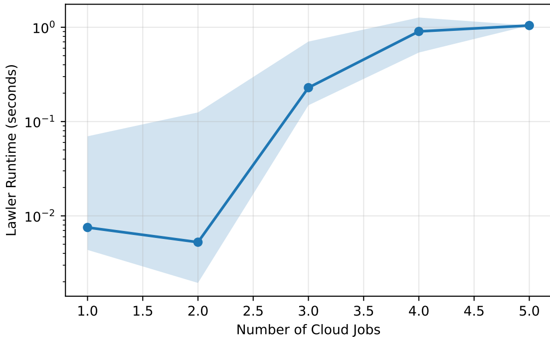
Cloud Jobs vs. Lawler Runtime
