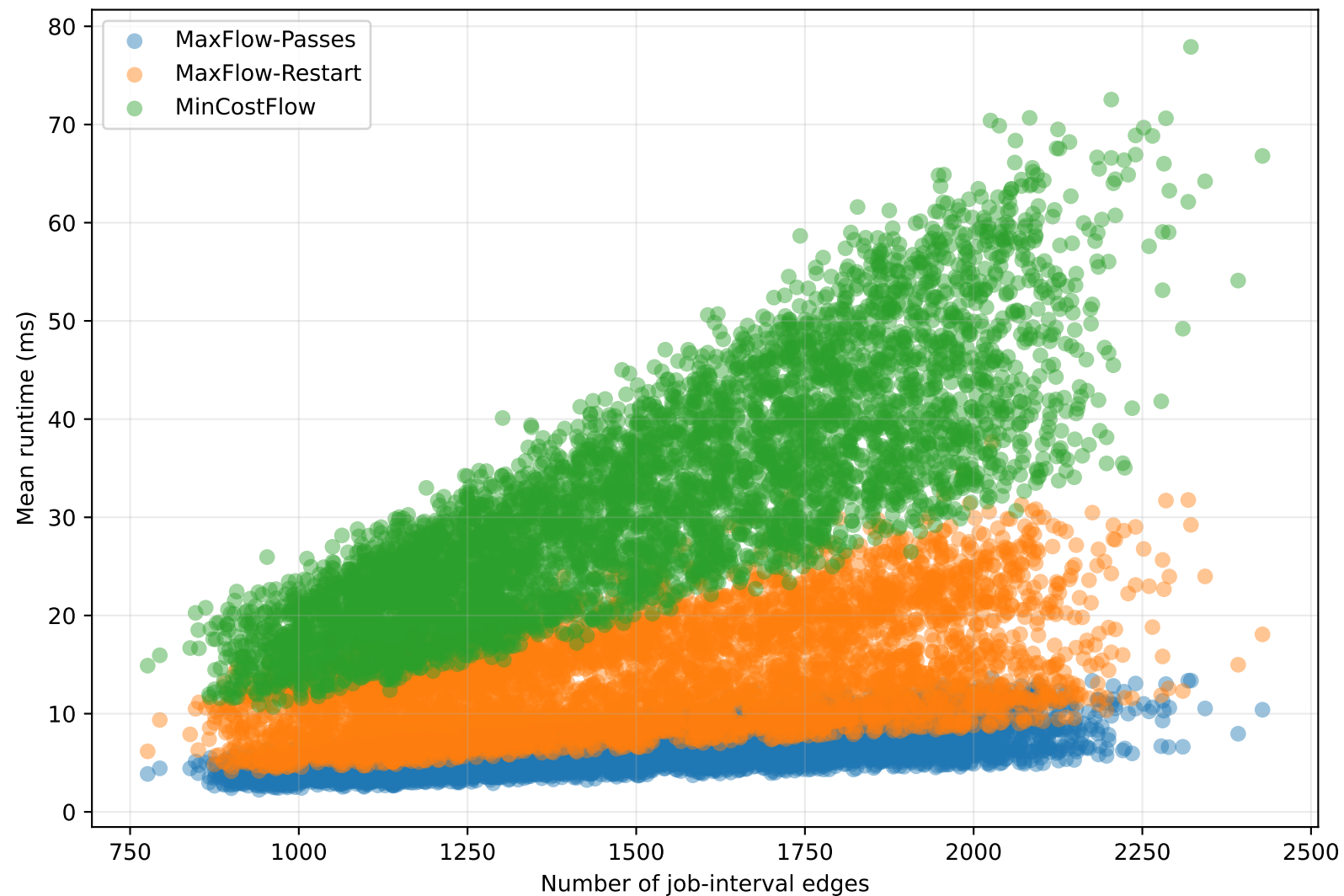
Runtime vs. Flow-Network Size
