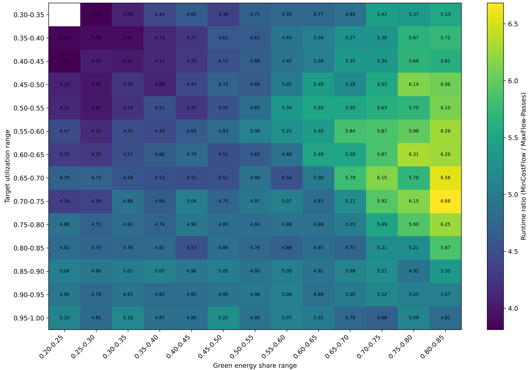
Runtime Ratio: Pure Min-Cost Flow / MaxFlow-Passes
