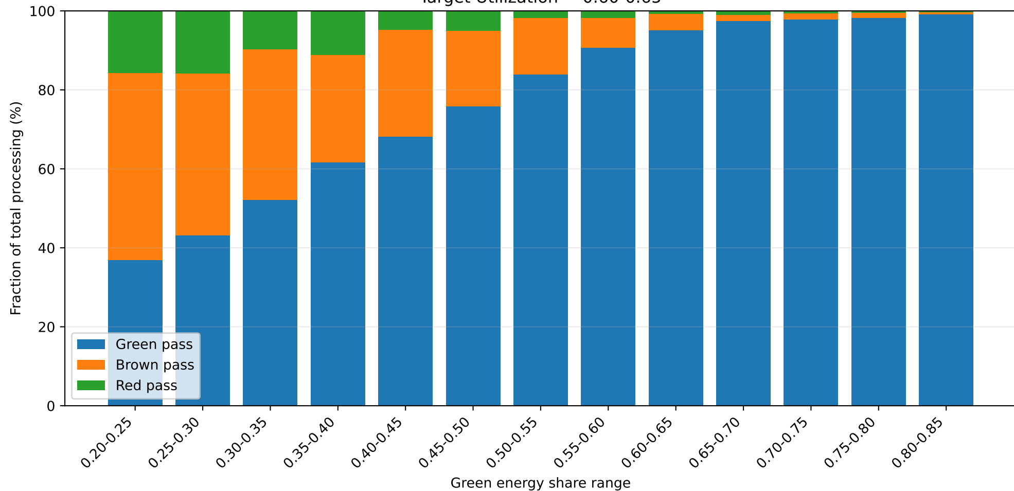
Flow Introduced by Each Max-Flow Phase Target Utilization = 0.60-0.65
