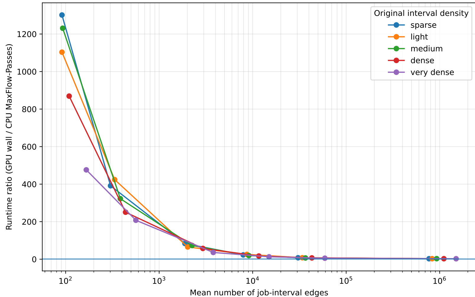
GPU wall time / CPU MaxFlow-Passes vs. network size
