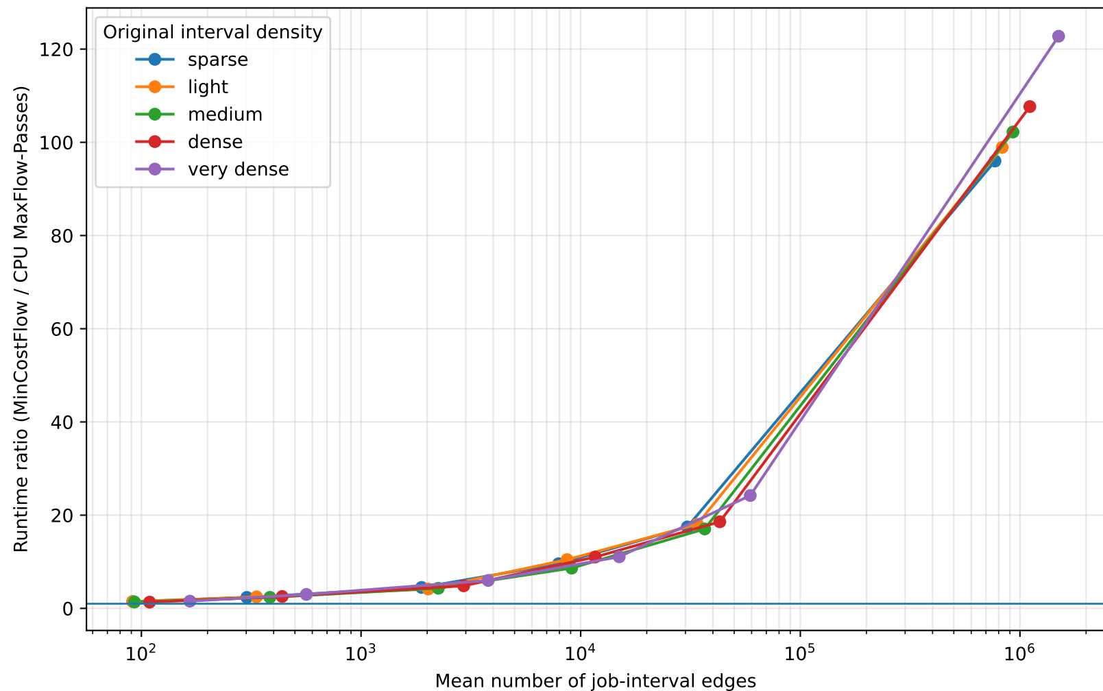
MinCostFlow / CPU MaxFlow-Passes vs. network size
