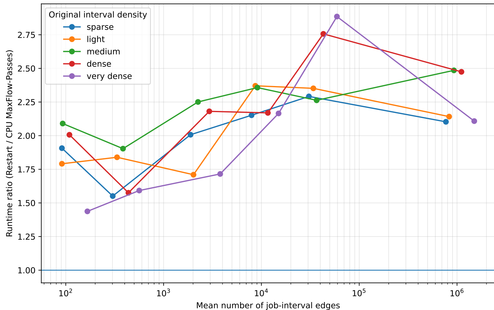
MaxFlow-Restart / CPU MaxFlow-Passes vs. network size
