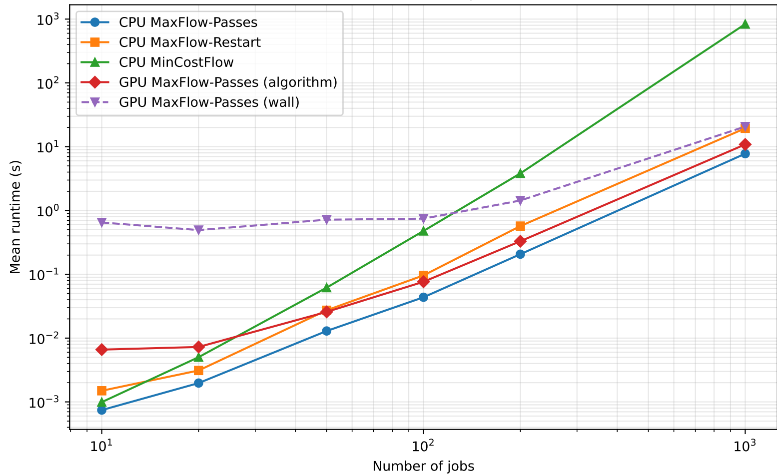
Exact-solver scalability — dense
