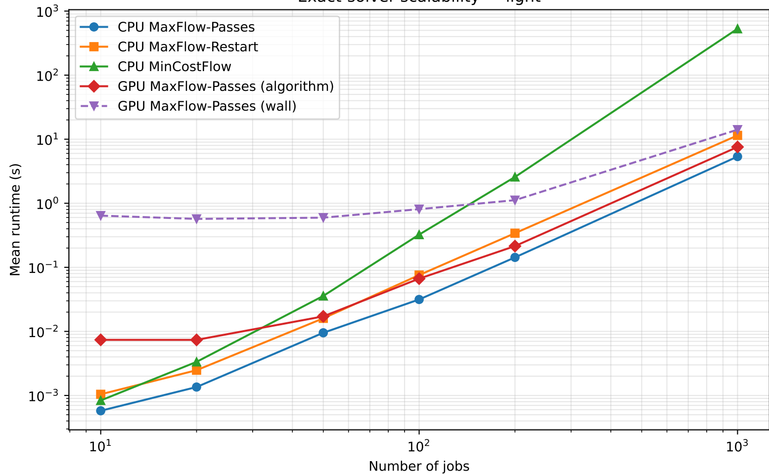
Exact-solver scalability — light
