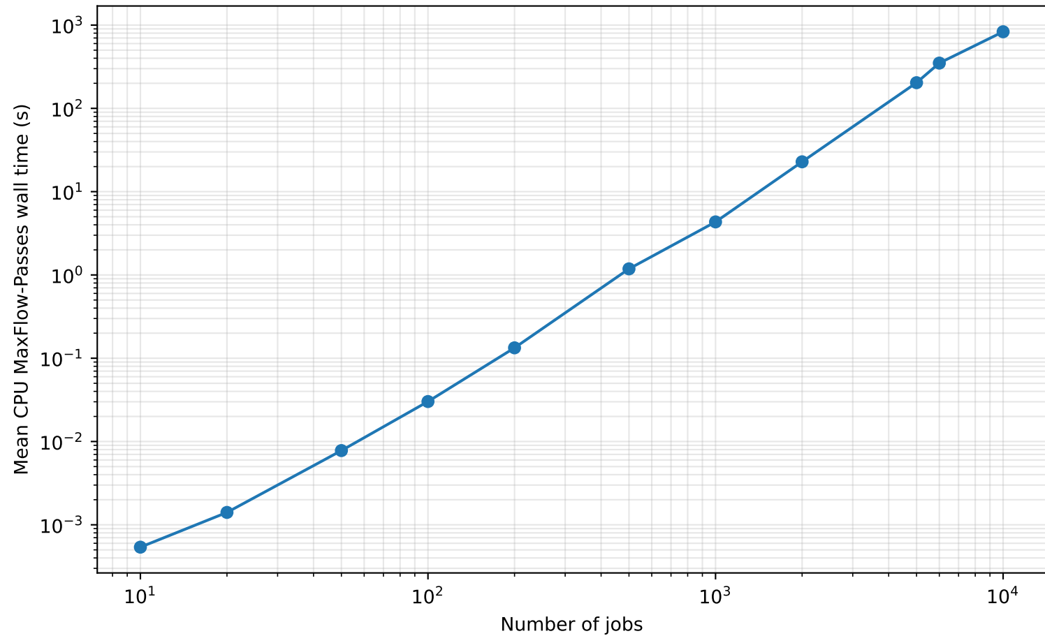
CPU MaxFlow-Passes — light intervals
