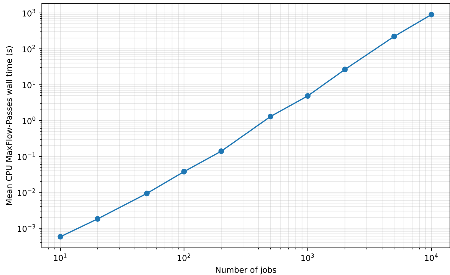
CPU MaxFlow-Passes — medium intervals
