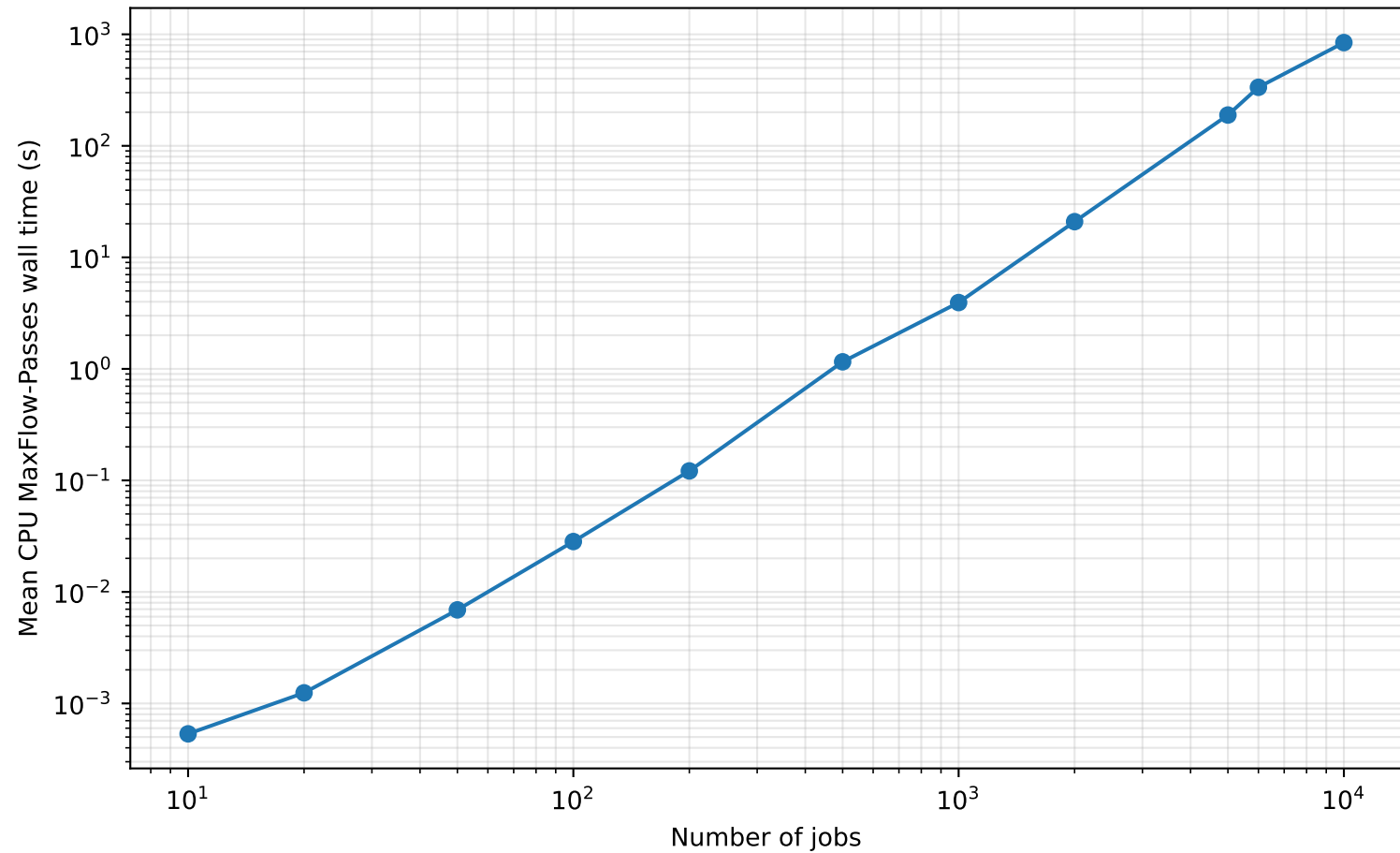
CPU MaxFlow-Passes — sparse intervals
