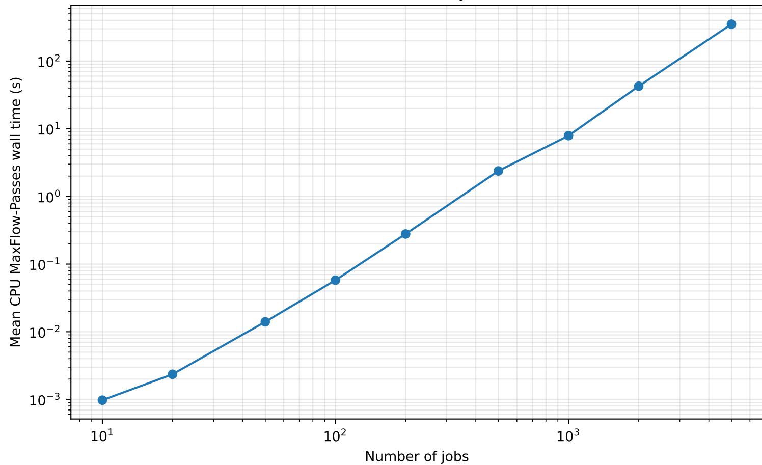
CPU MaxFlow-Passes — very dense intervals
