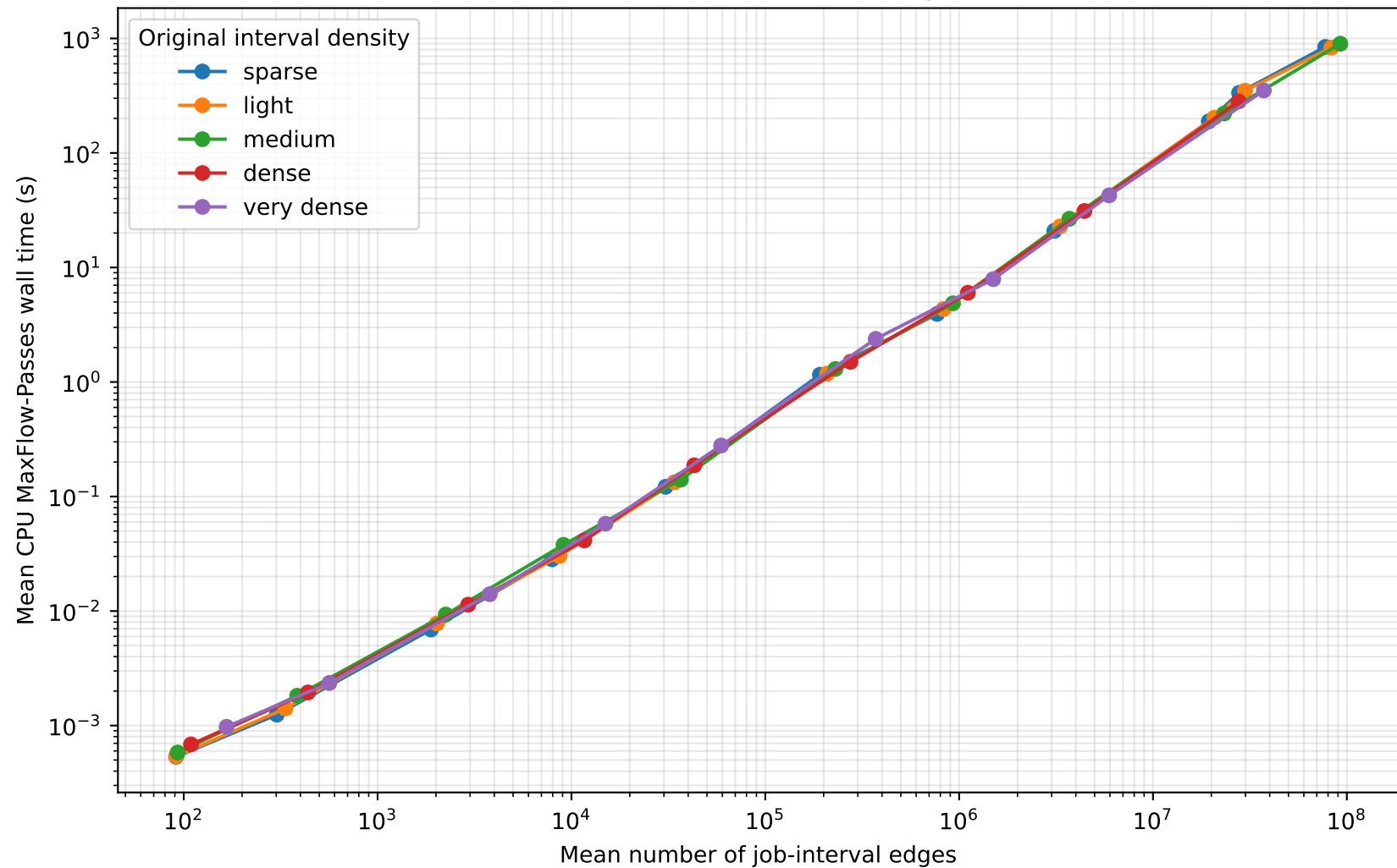
CPU runtime vs. flow-network edge count
