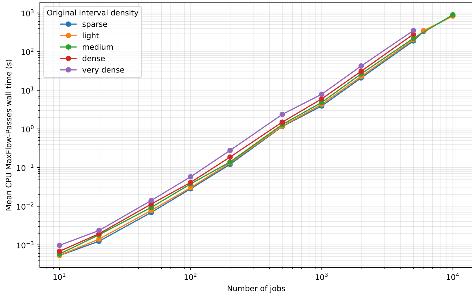
CPU MaxFlow-Passes scalability
