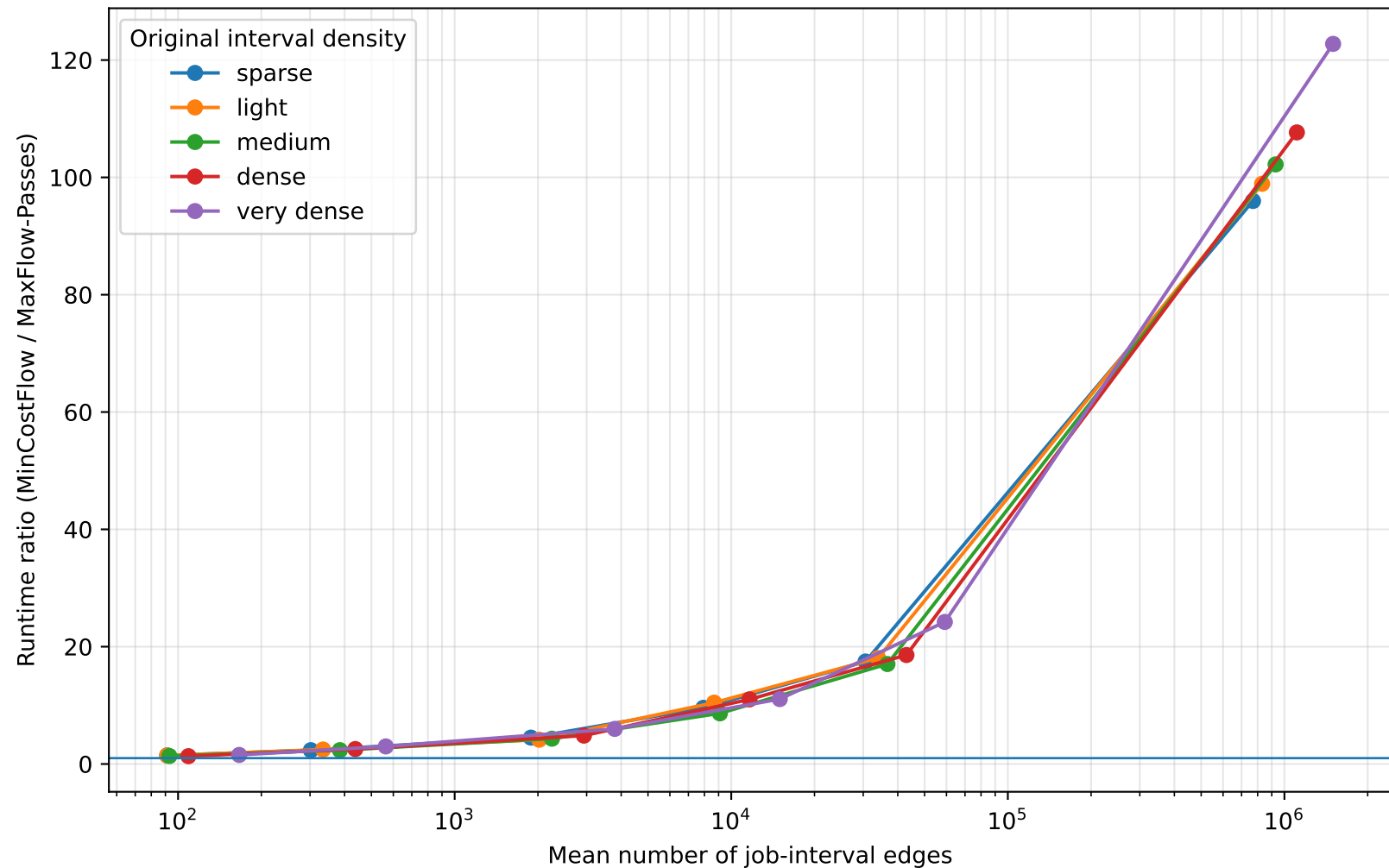
MinCostFlow / MaxFlow-Passes vs. network size
