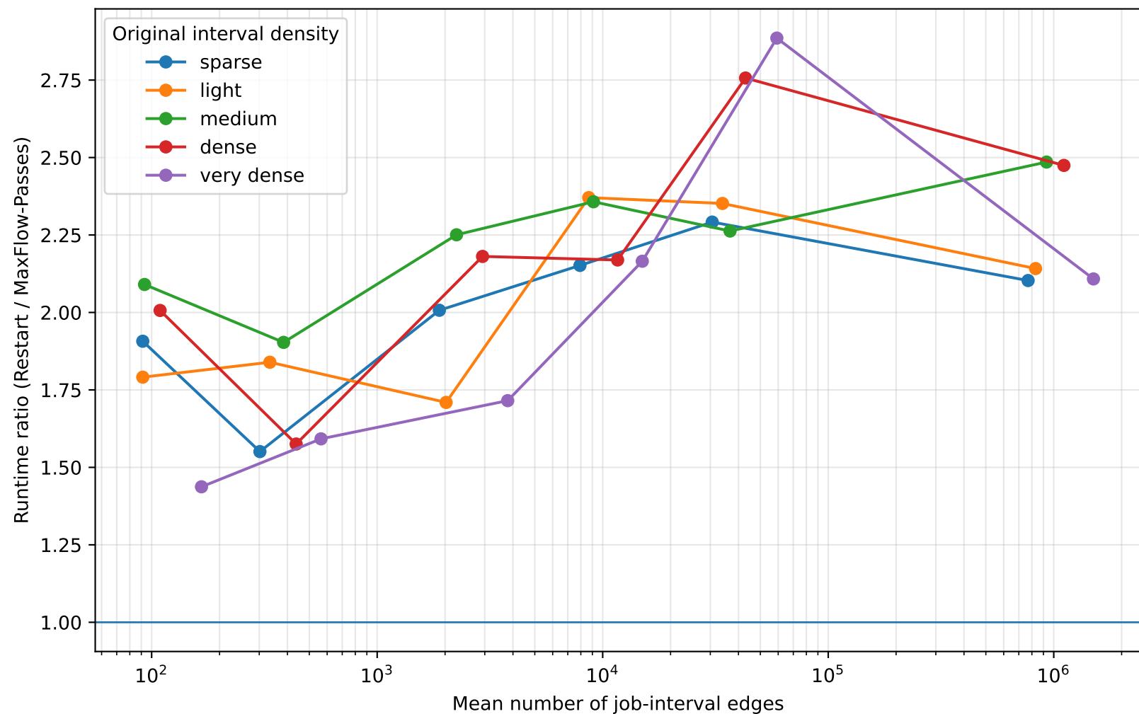
MaxFlow-Restart / MaxFlow-Passes vs. network size
