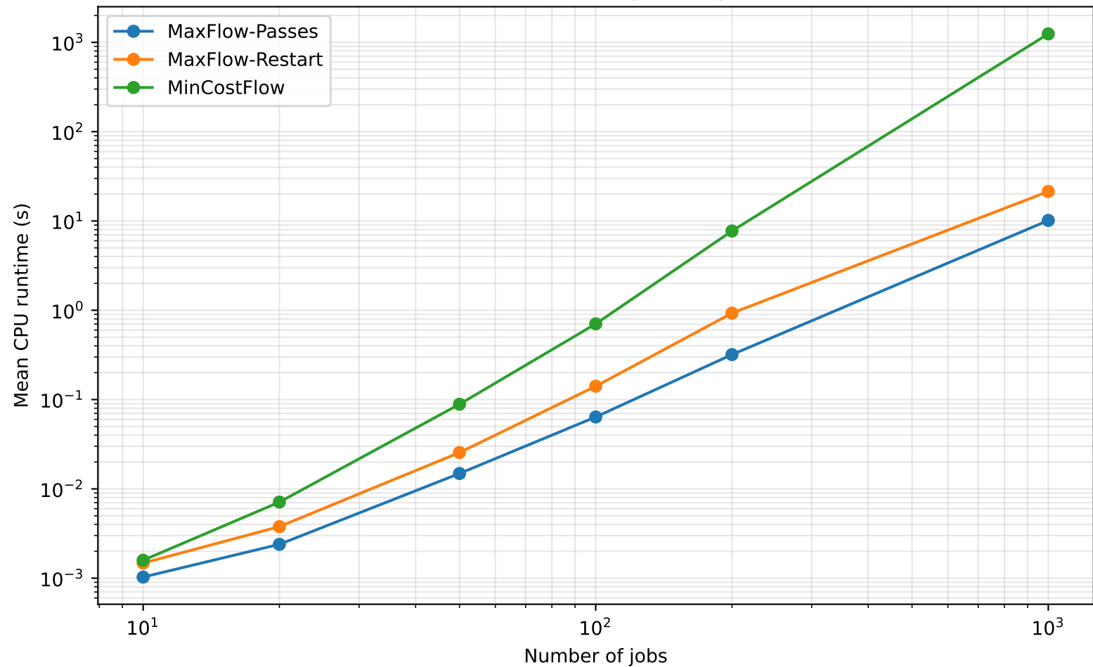
Exact-solver scalability — very dense
