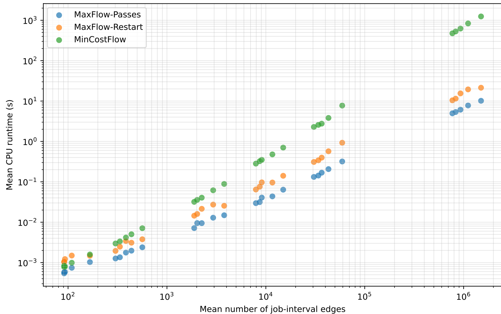
Exact-solver runtime vs. flow-network size
