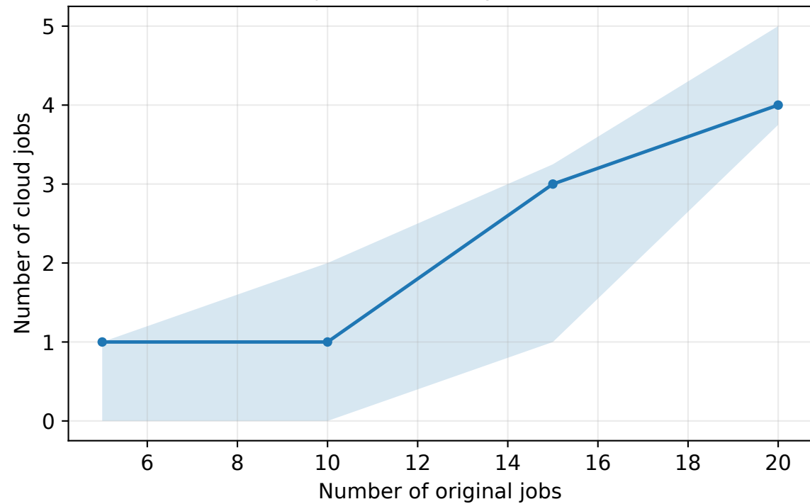
Cloud job count vs. problem size
