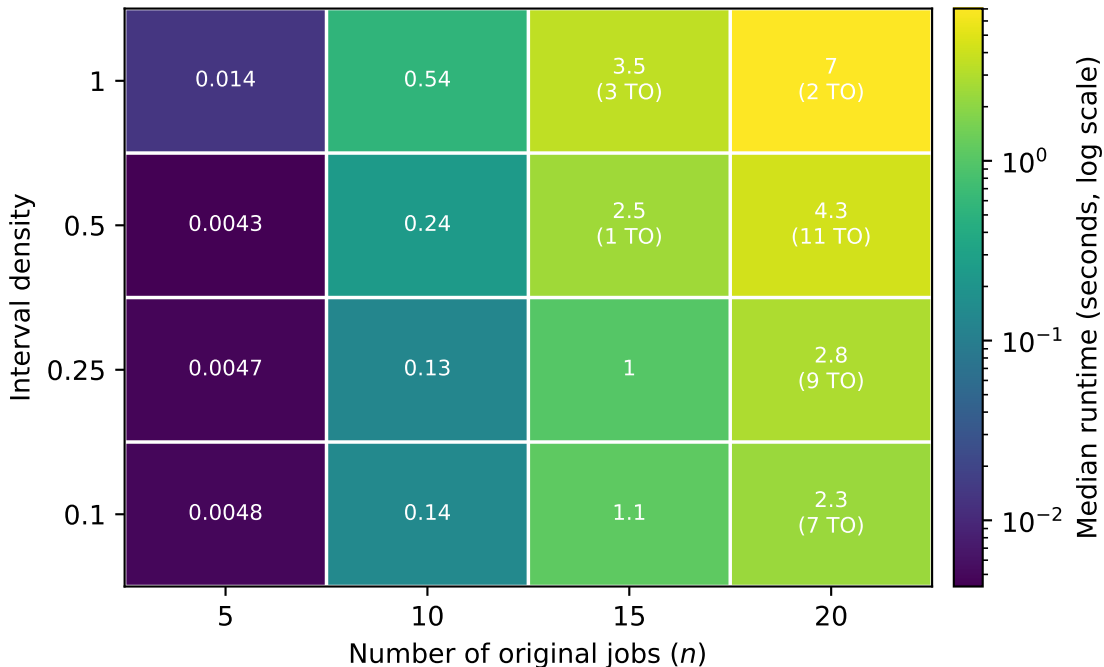
Lawler runtime by jobs and interval density
