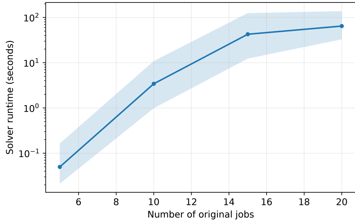
Lawler runtime scaling
