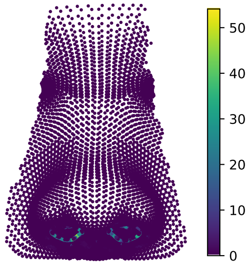
New-flip frequency (%)
