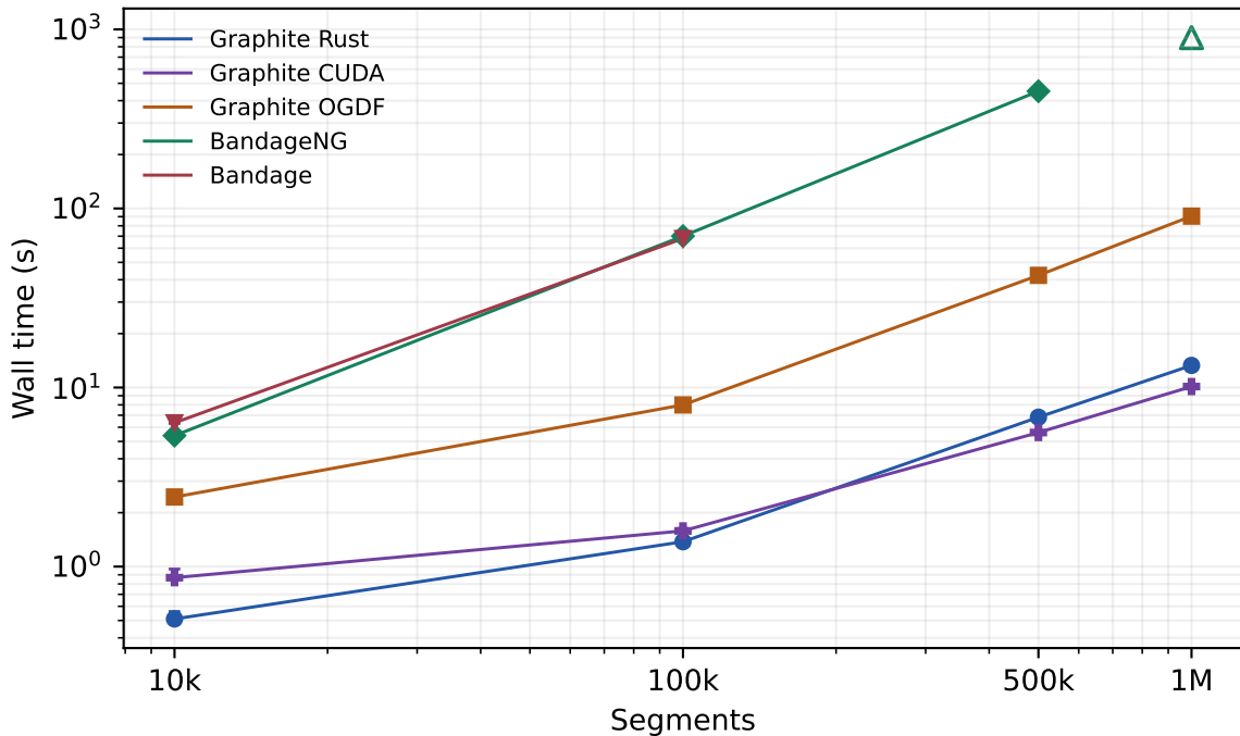
Branched synthetic graphs
