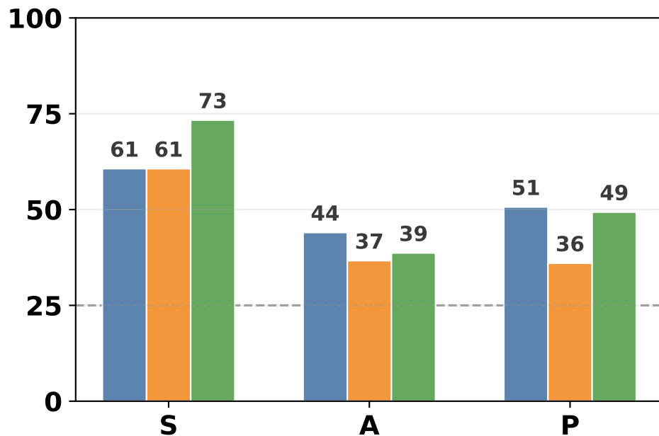
Qwen3.5-397B
