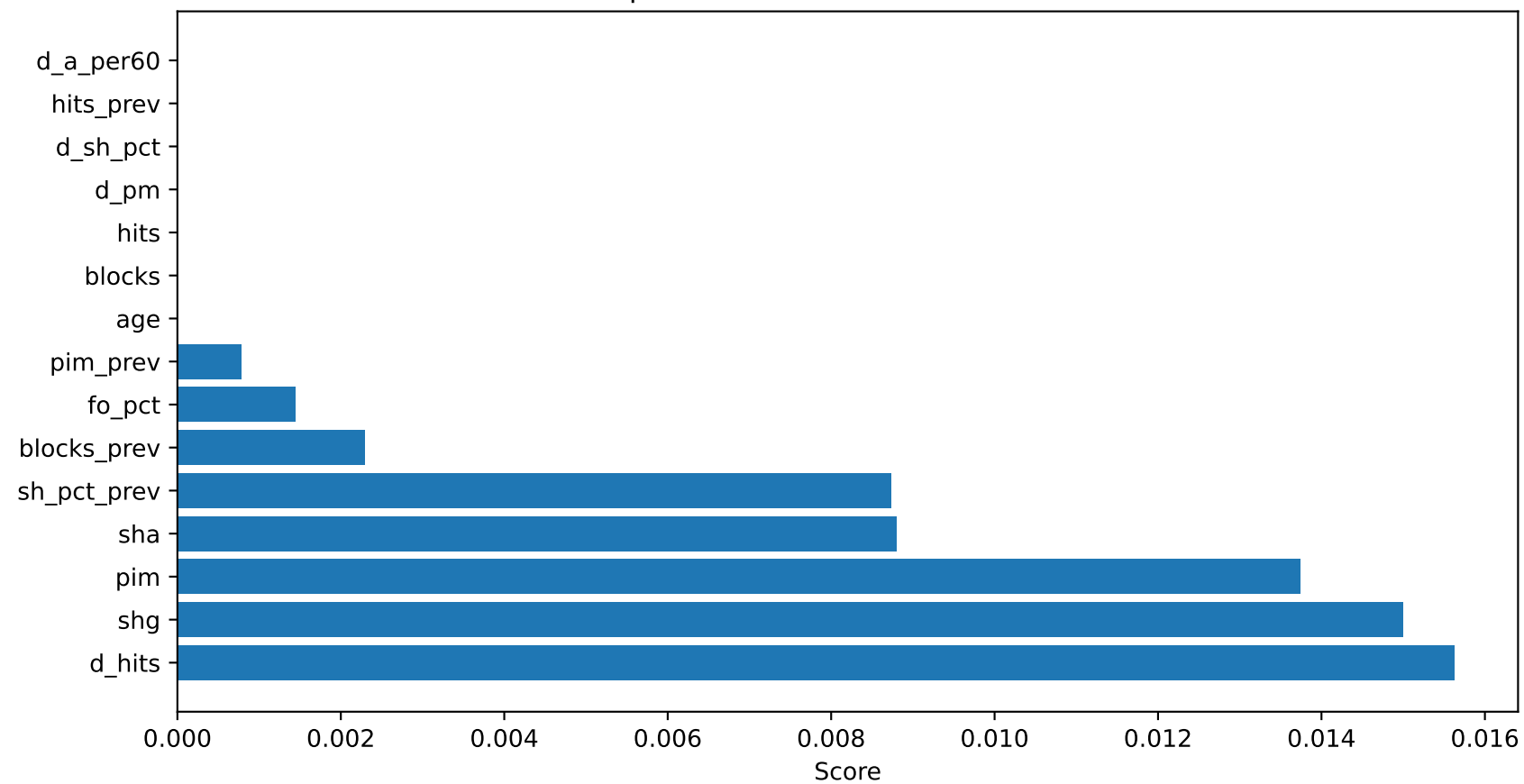
Top features — Mutual information
