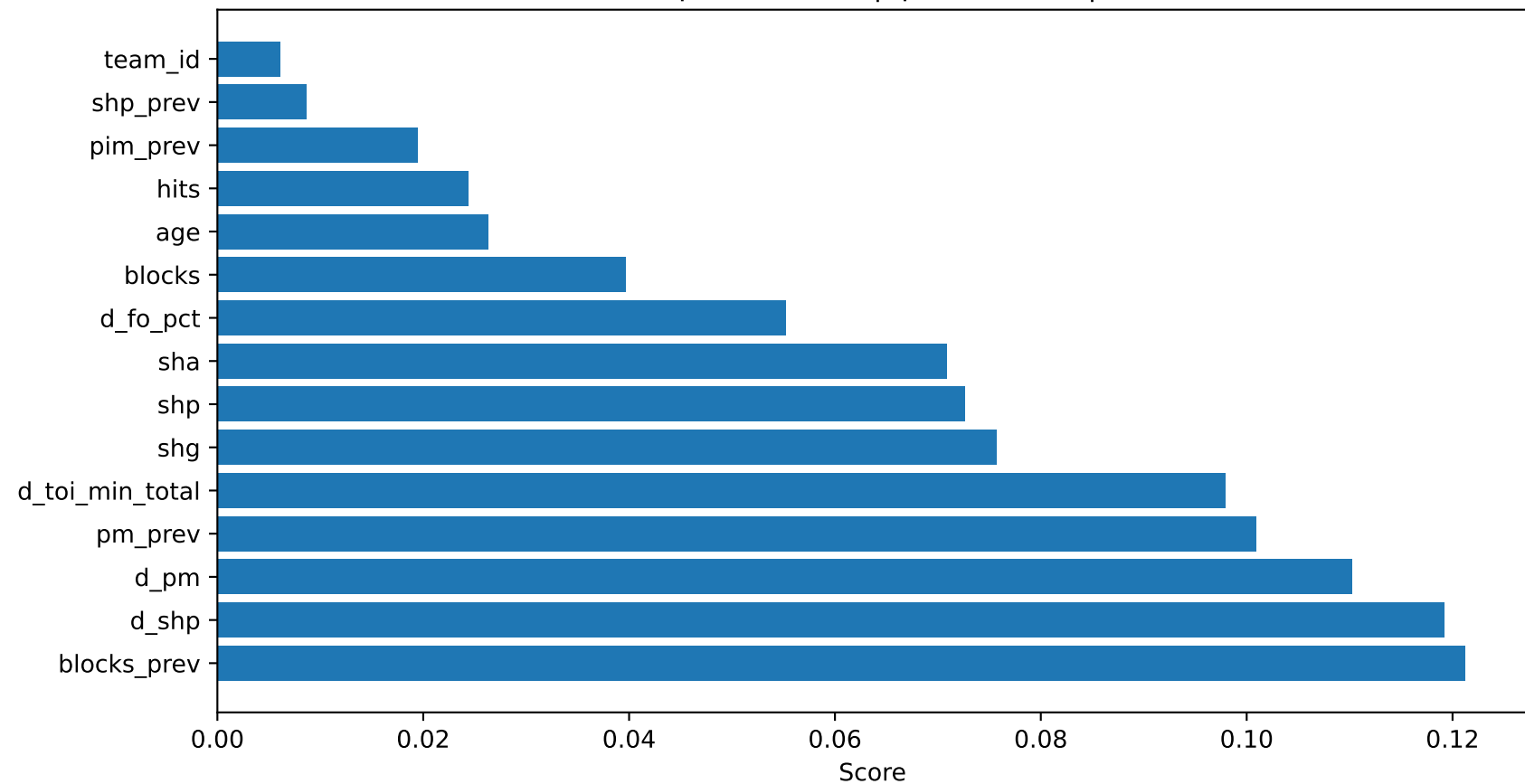
Top features — |Spearman rho|
