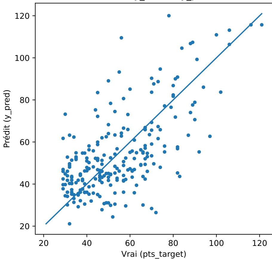
TEST — y_{\text{true}} vs y_{\text{pred}}
