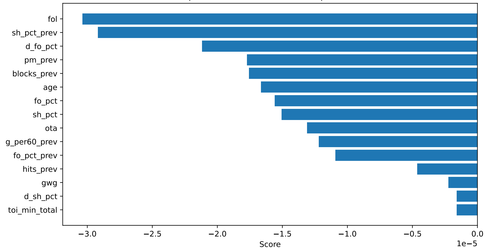
Top features — Permutation importance
