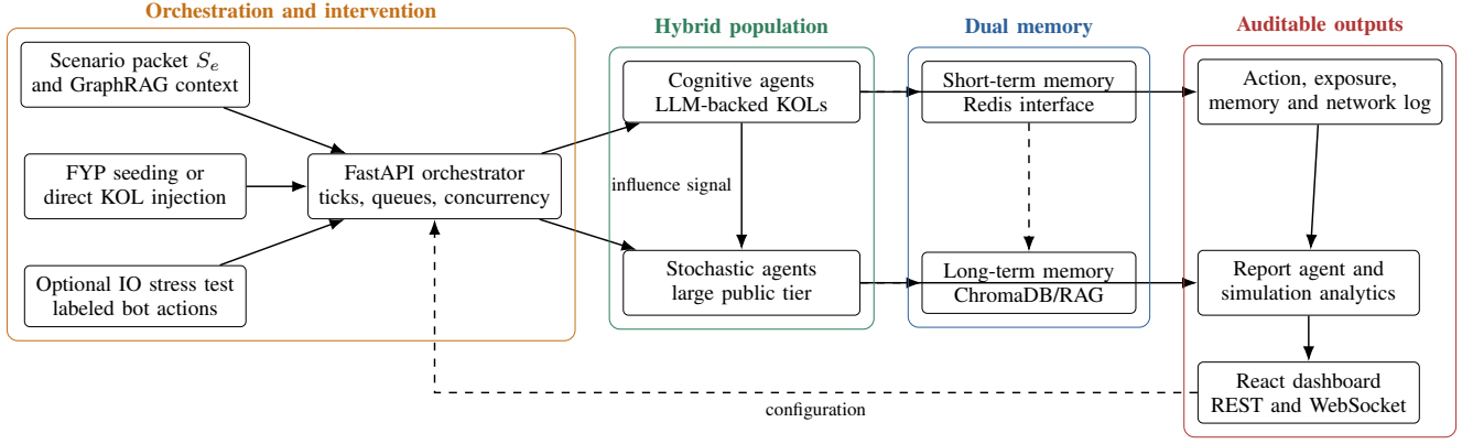
Fig. 2. DEEDY Simulation Core architecture. The core is MiroFish-based and its hybrid-ABM and dual-memory design is informed by the ISAL-NLP MarketFish manuscript [18]. The orchestrator combines configurable exposure and intervention with a hybrid cognitive–stochastic population; agents use short- and long-term memory, and their traces feed reporting and the live application. Solid arrows denote the main execution/data path; dashed arrows denote memory or configuration access.
