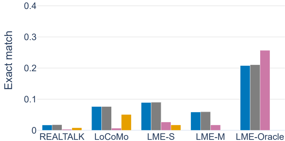
Exact match
