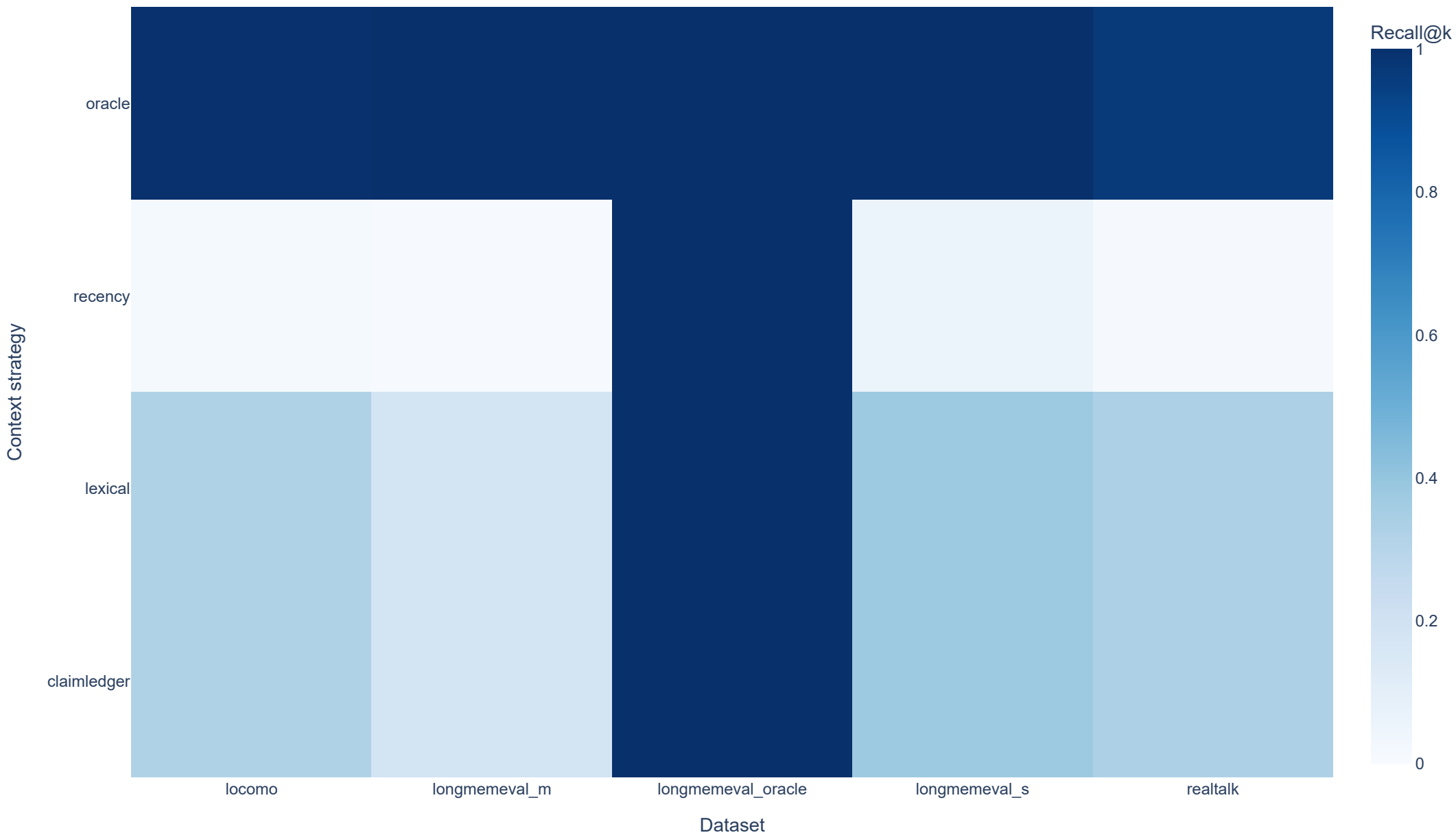
Evidence recall across official benchmark releases
