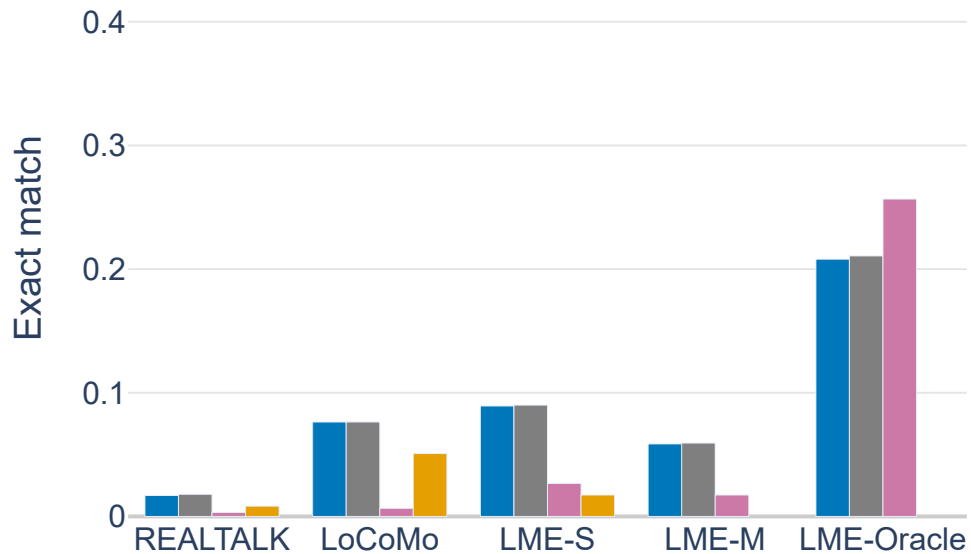
Exact match
