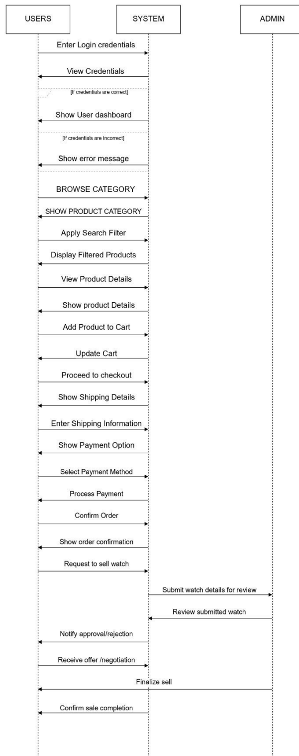
Figure. 4.1 Sequence Diagram
