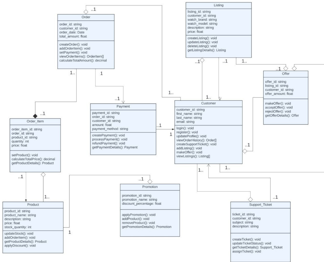
Figure. 3.1 Class Diagram
