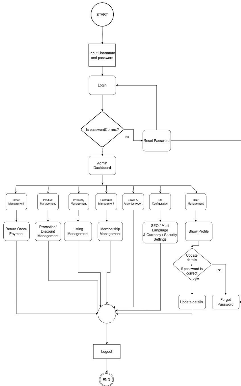
Figure. 1.1 Admin Activity
