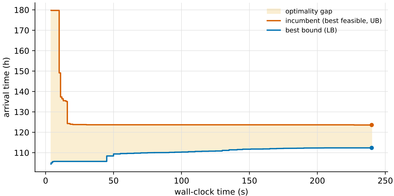
Oracle MIP bound evolution — RlongCfewTlarge_12 N=181 stops, status=maxTimeLimit, final gap 9.08%
