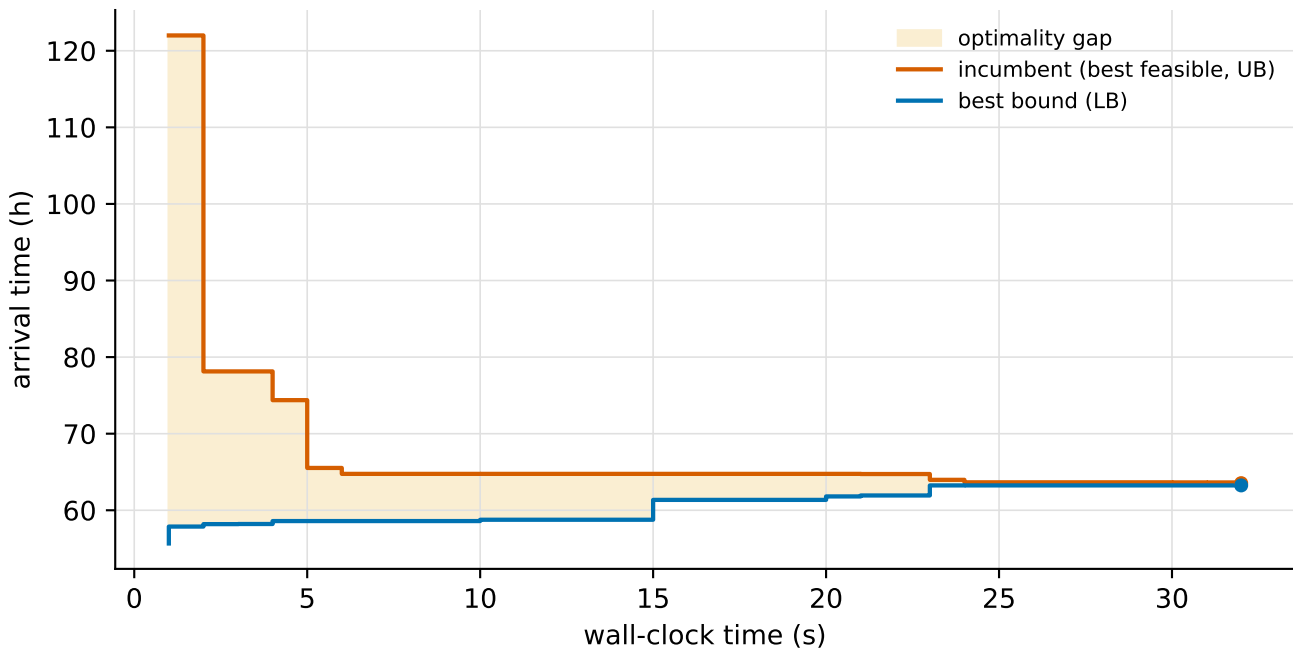
Oracle MIP bound evolution — RmediumCfewTlarge_1 N=104 stops, status=optimal, final gap 0.47%
