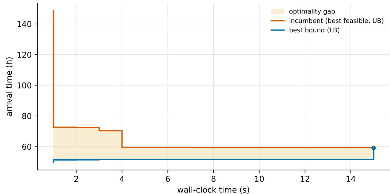
Oracle MIP bound evolution — RmediumCfewTlarge_2 N=89 stops, status=optimal, final gap 0.47%
