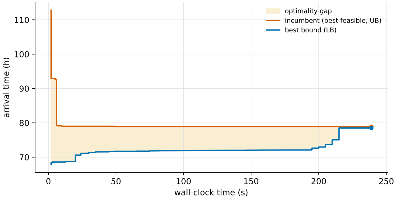
Oracle MIP bound evolution — RmediumCfewTlarge_3 N=124 stops, status=optimal, final gap 0.49%
