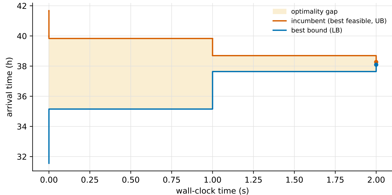
Oracle MIP bound evolution — RshortCfewTlarge_1 N=61 stops, status=optimal, final gap 0.46%
