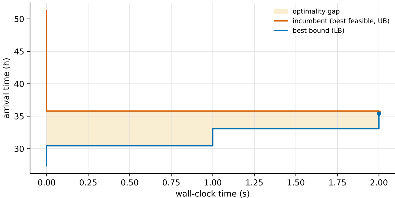
Oracle MIP bound evolution — RshortCfewTlarge_3 N=52 stops, status=optimal, final gap 0.49%
