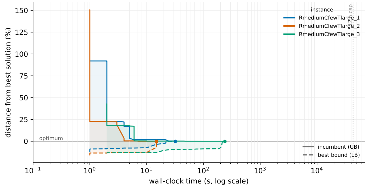
Medium routes — oracle bound convergence (n=3) upper = incumbent, lower = best bound
