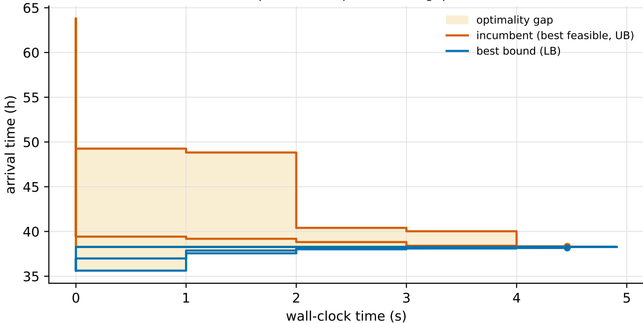
Oracle MIP bound evolution — RshortCfewTlarge_1 N=61 stops, status=optimal, final gap 0.47%
