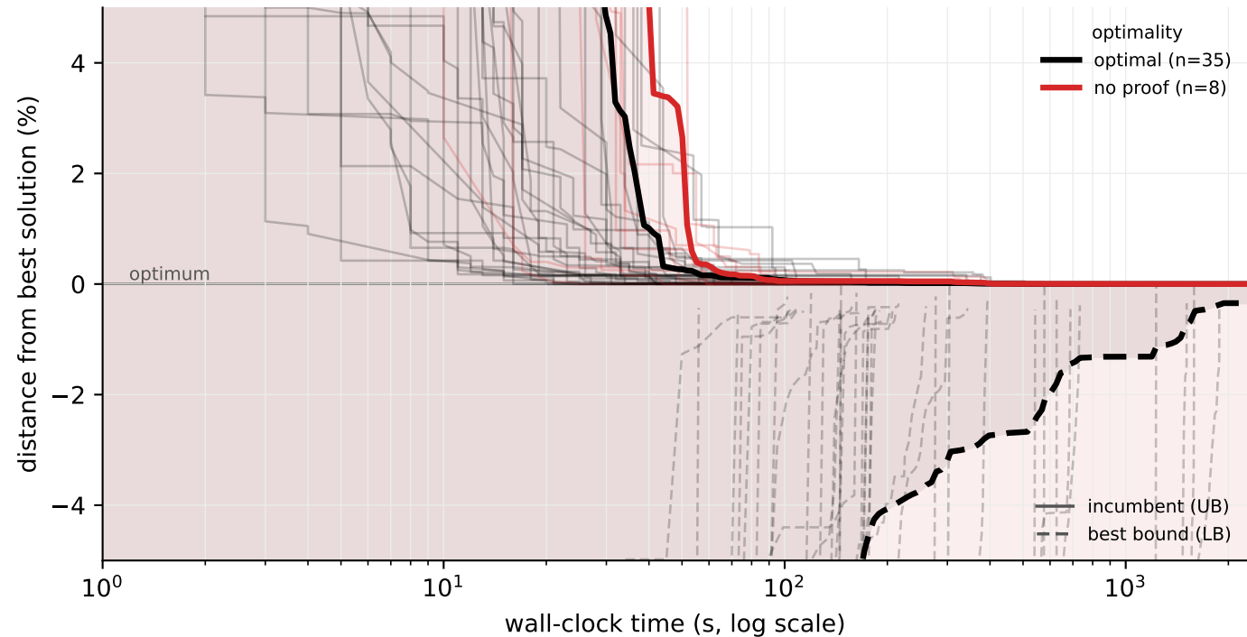
Medium routes — oracle bound convergence (n=43) black = optimal, red = no proof (bold = group average, faded = instances)
